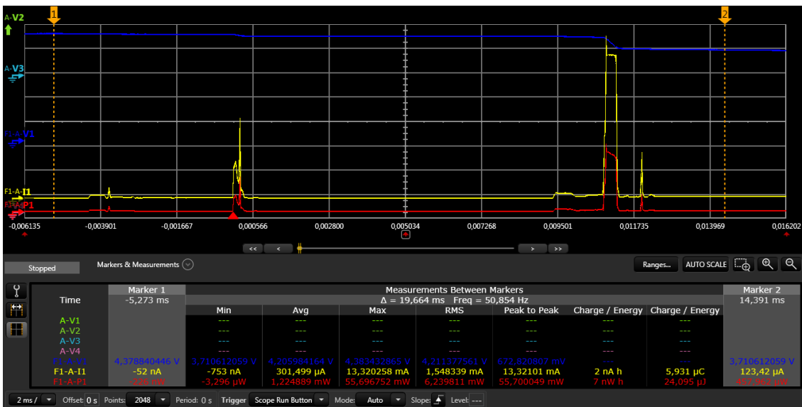
Fig. 8. 10μF storage. Frame is enough for Ble. 1 ADV sent /1v/div, 2mA/div, 20mw/div). Whole system starts around 4.4V and works down to 3.7 volts. 24μJ measured.
